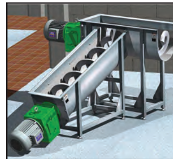
Martin Sprocket Screw Conveyor
